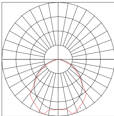
Midibay Pro - 110 degree distribution
