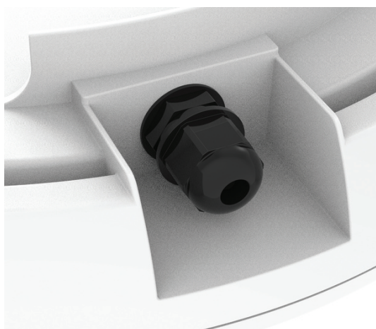
Cable Entry Gland (15W Pictured)
